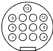
VIEW INTO BACK OF RADIO (INTO BACK OF PLUG)
